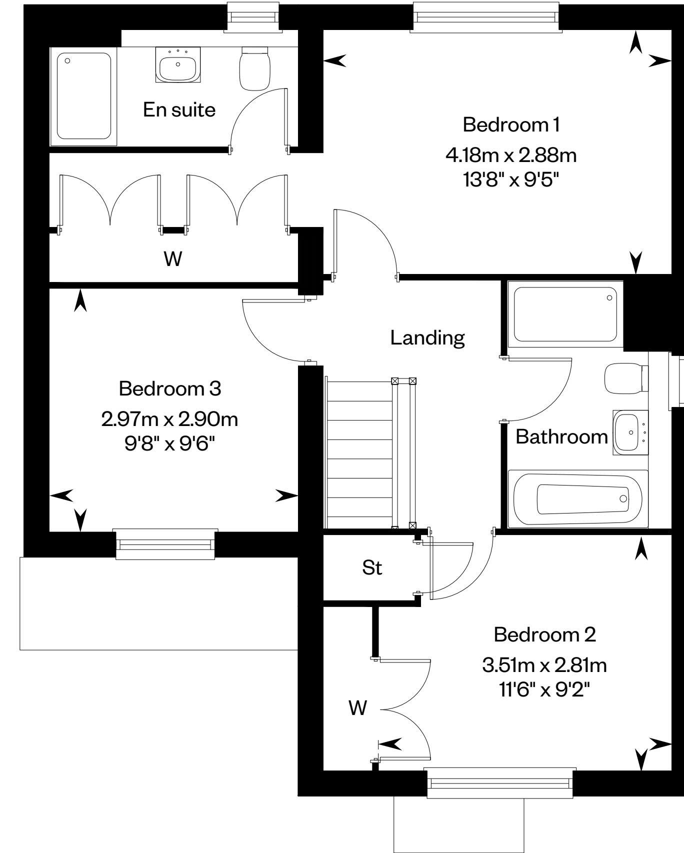
First floor
