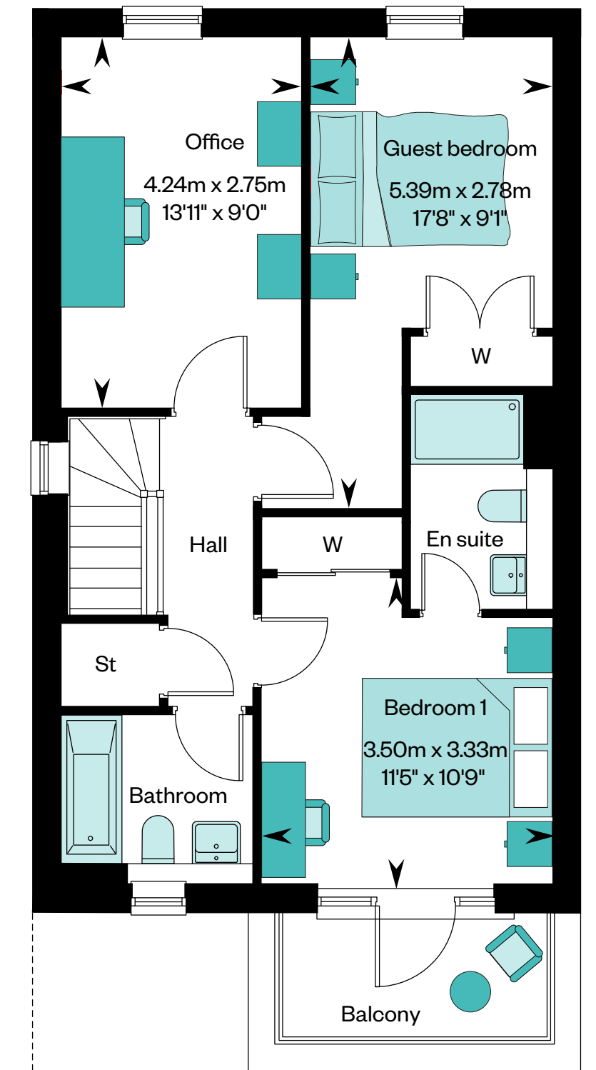
First floor
