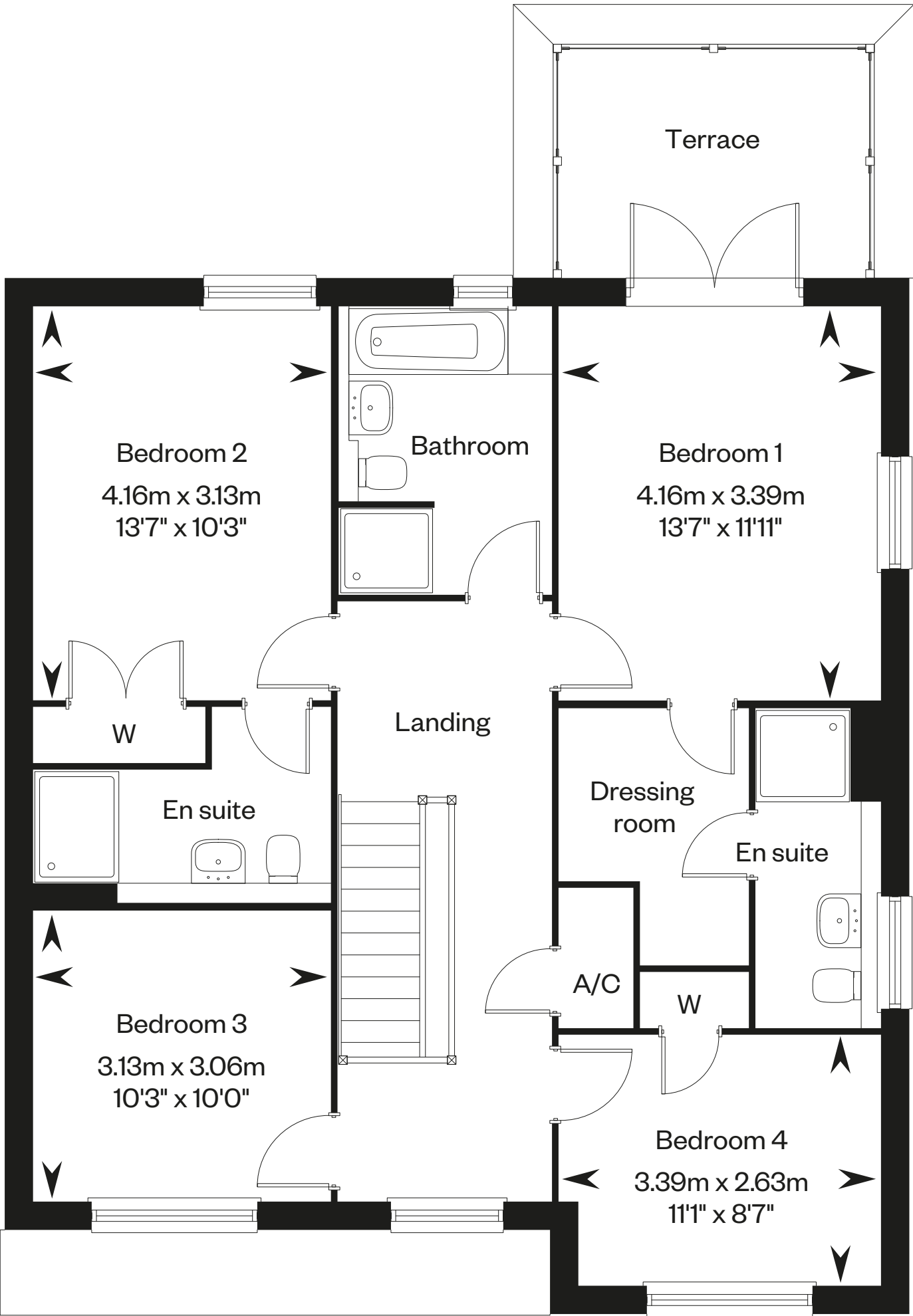
First floor
