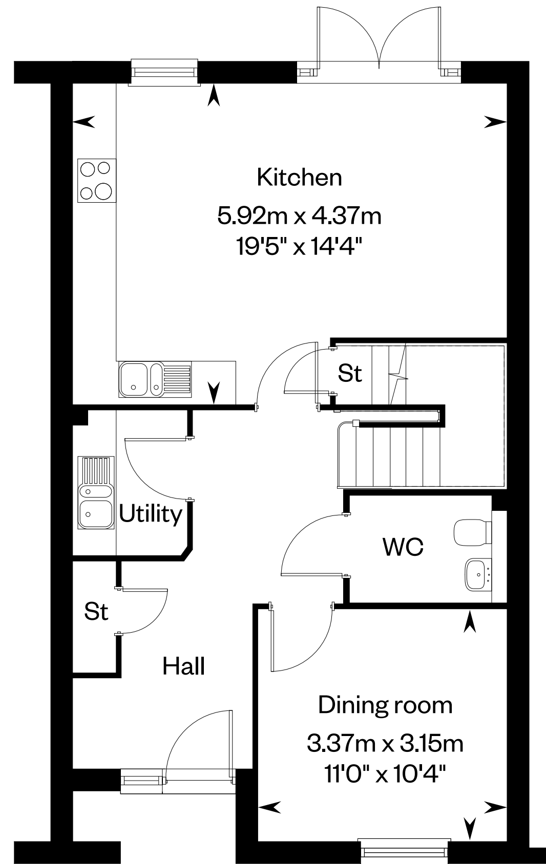
Ground floor
