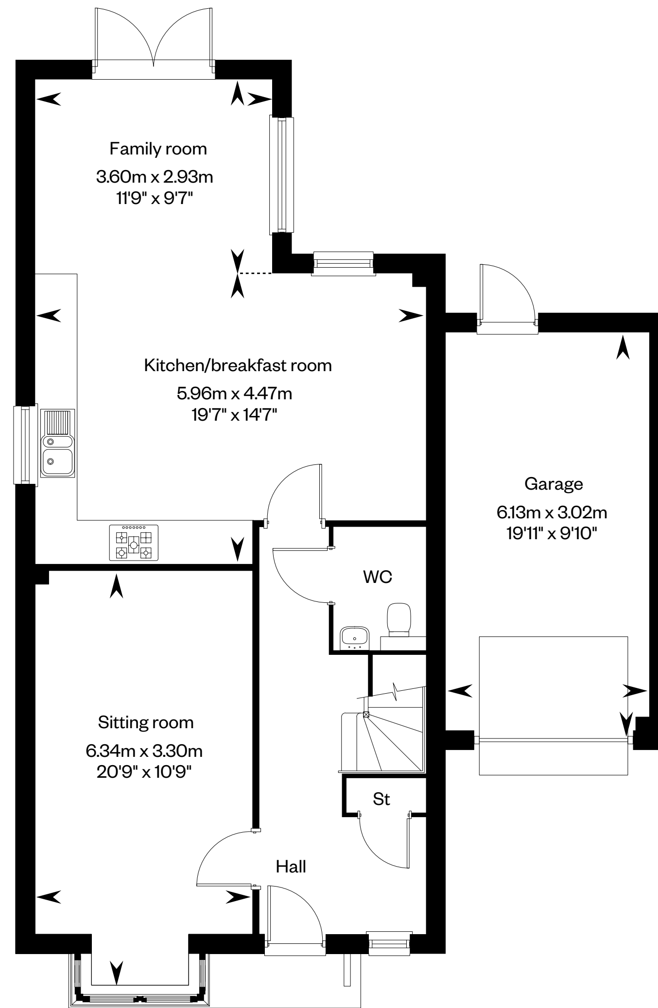
Ground floor
