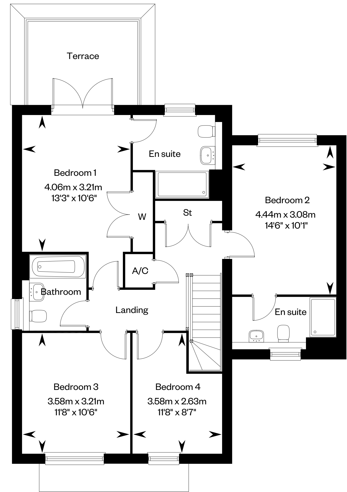
First floor
